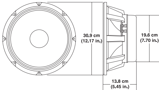
FIGURE 5 — Dimensions
