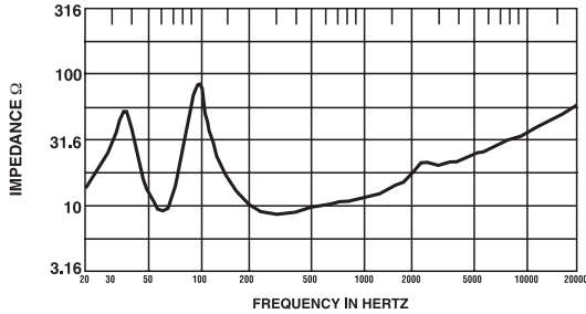
FIGURE 4 — Impedance in Typical Enclosure (2.0 ft 3 )
