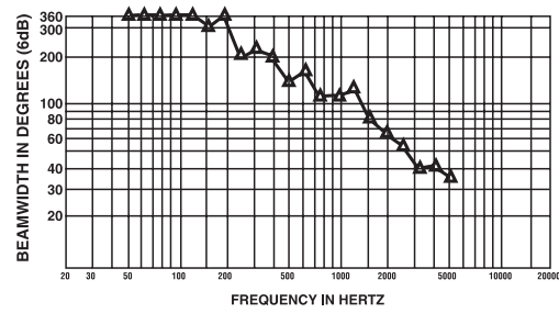
FIGURE 8 — Directivity vs. Frequency
