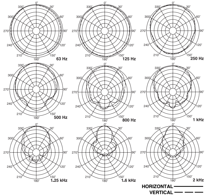
FIGURE 9 — Polar Response
