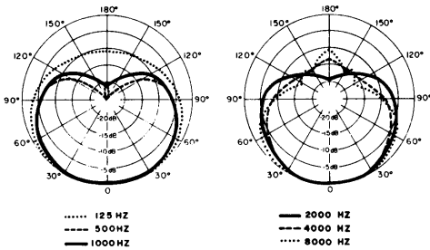
TYPICAL POLAR PATTERNS FIGURE 3
